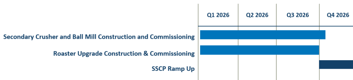
Figure 10: SSCP Timeline
